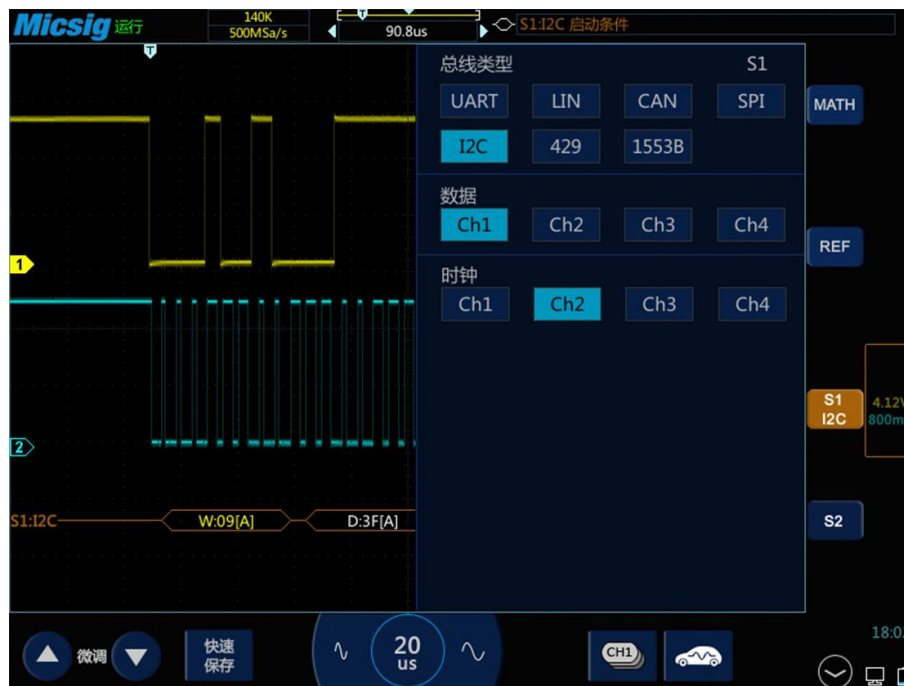
图14-21 I2C 总线配置菜单
