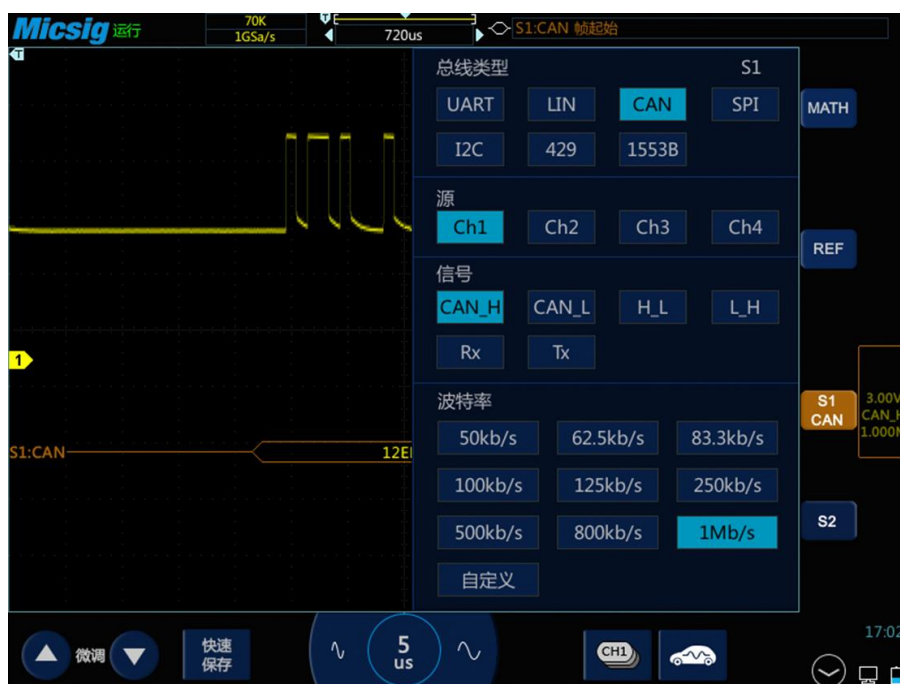
图14-13 CAN 总线配置菜单
