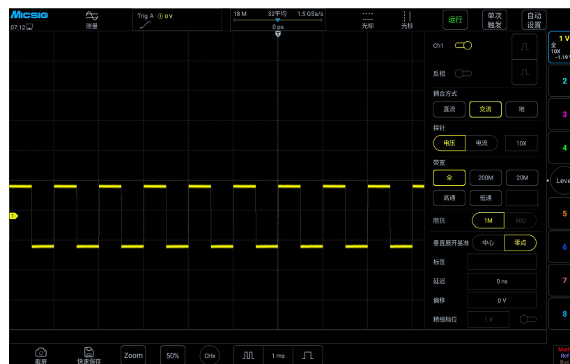
图5-8 AC耦合
