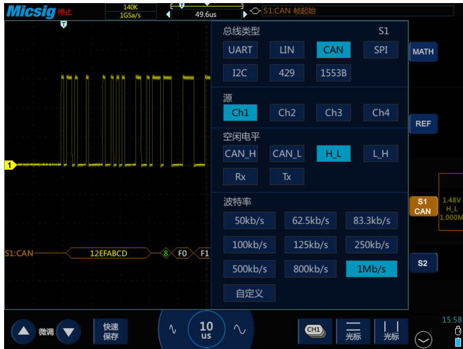
图13-13 CAN 总线配置菜单
