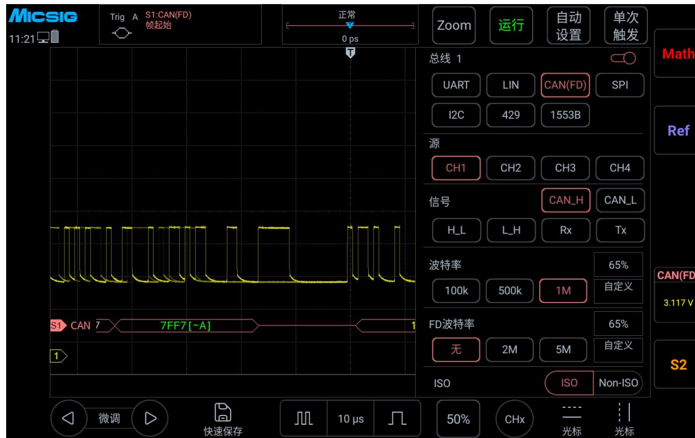
图 14-14 CAN / CAN FD 总线配置菜单
