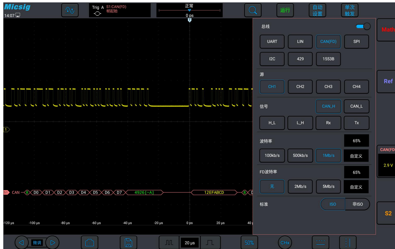
图 12-14 CAN / CAN FD 总线配置菜单
